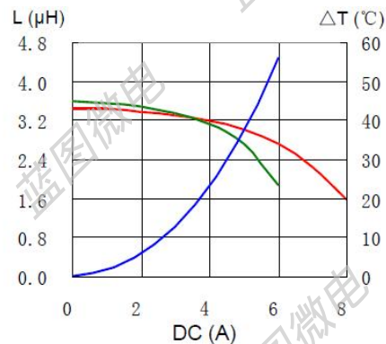
SRH8D38-100N
