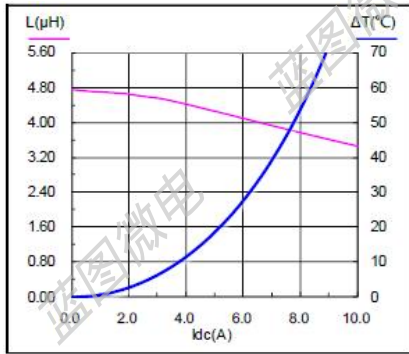
SMS0650-100M
