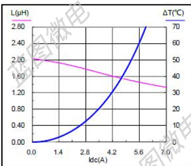
SMS0520-5R6M
