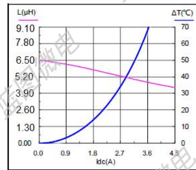
SMS0520-6R8M
