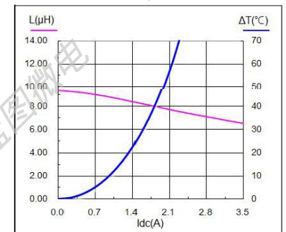
SMS0520-100M
