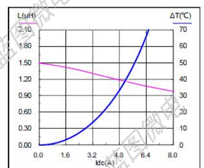
SMS0520-1R5M
